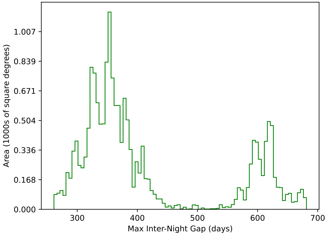
too_elab_r8_d3_ugrizy_v3.4_10yrs WFD g band: Max Inter-Night Gap
