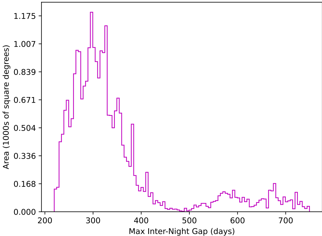
too_elab_r8_d3_ugrizy_v3.4_10yrs All sky z band: Max Inter-Night Gap
