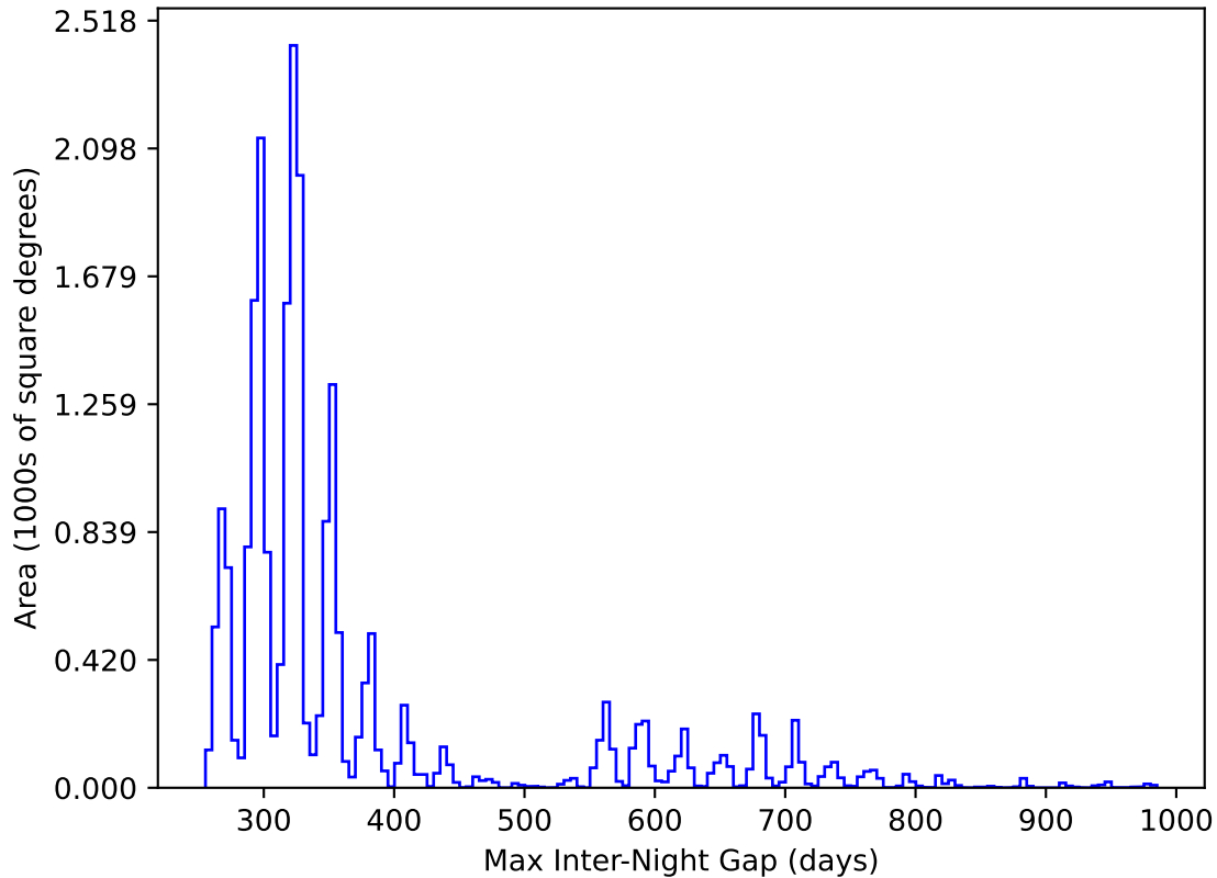
too_elab_r8_d3_ugrizy_v3.4_10yrs All sky y band: Max Inter-Night Gap
