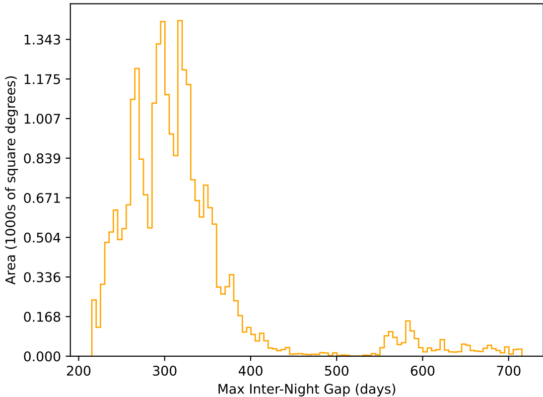
too_elab_r8_d3_ugrizy_v3.4_10yrs All sky r band: Max Inter-Night Gap
