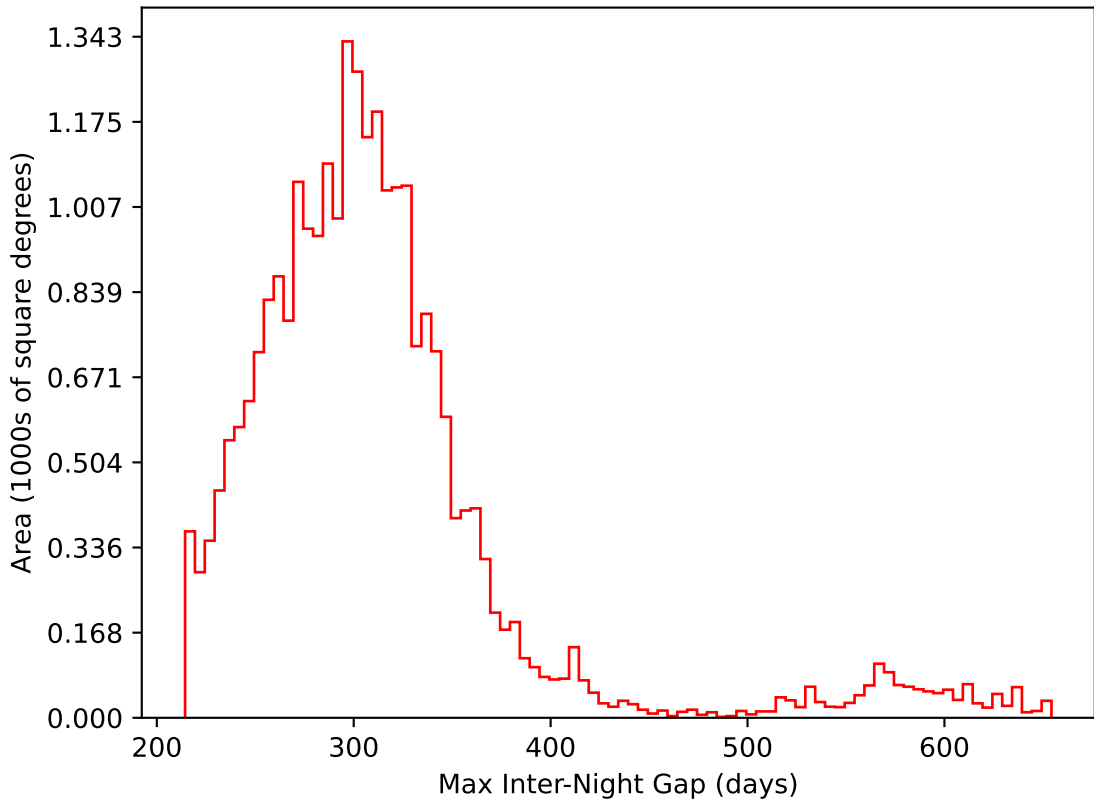
too_elab_r8_d3_ugrizy_v3.4_10yrs All sky i band: Max Inter-Night Gap
