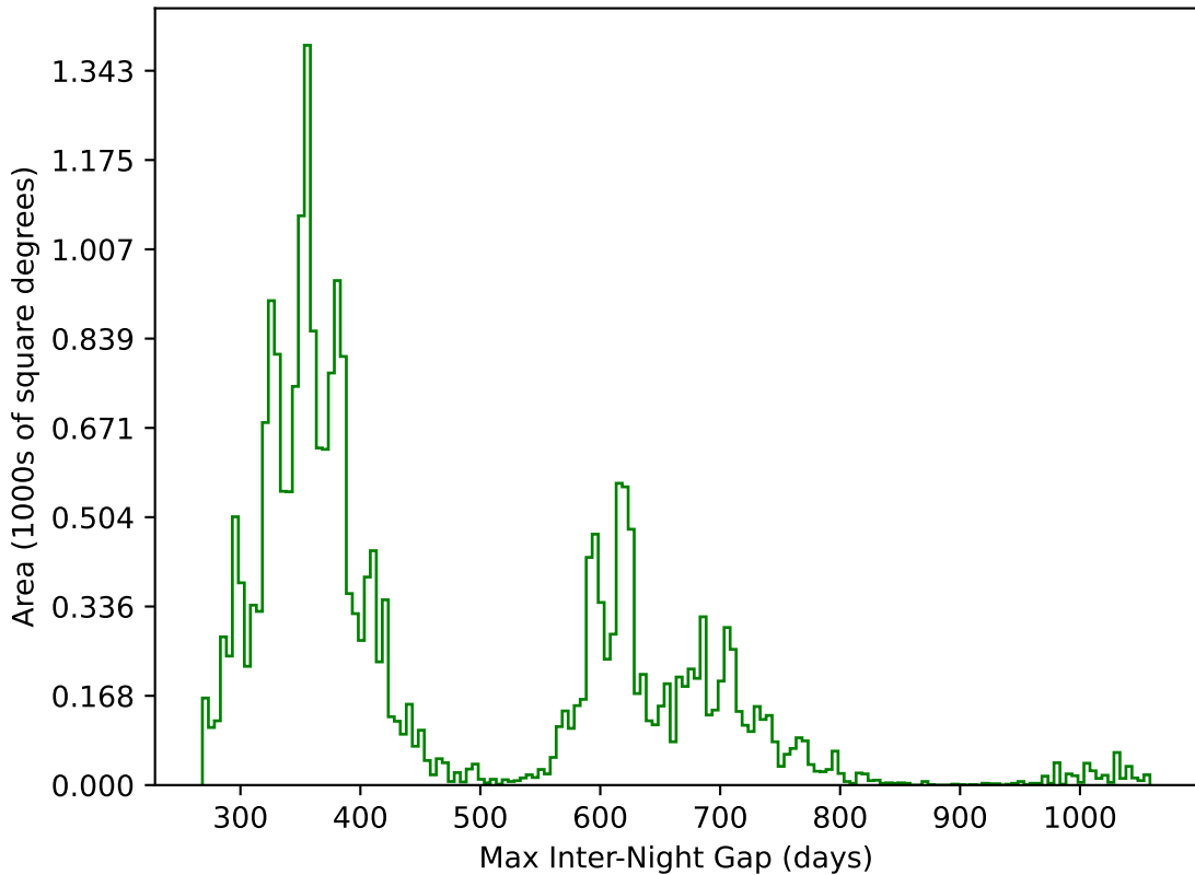
too_elab_r8_d3_ugrizy_v3.4_10yrs All sky g band: Max Inter-Night Gap
