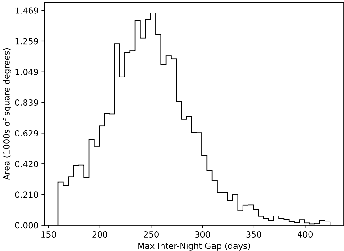
too_elab_r8_d3_ugrizy_v3.4_10yrs All sky all bands: Max Inter-Night Gap
