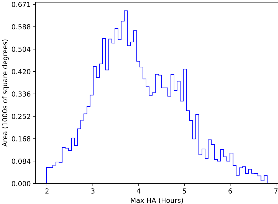
too_elab_r8_d3_ugrizy_v3.4_10yrs WFD u band: Max HA
