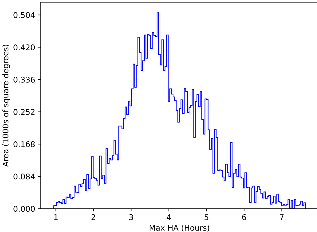
too_elab_r8_d3_ugrizy_v3.4_10yrs All sky u band: Max HA
