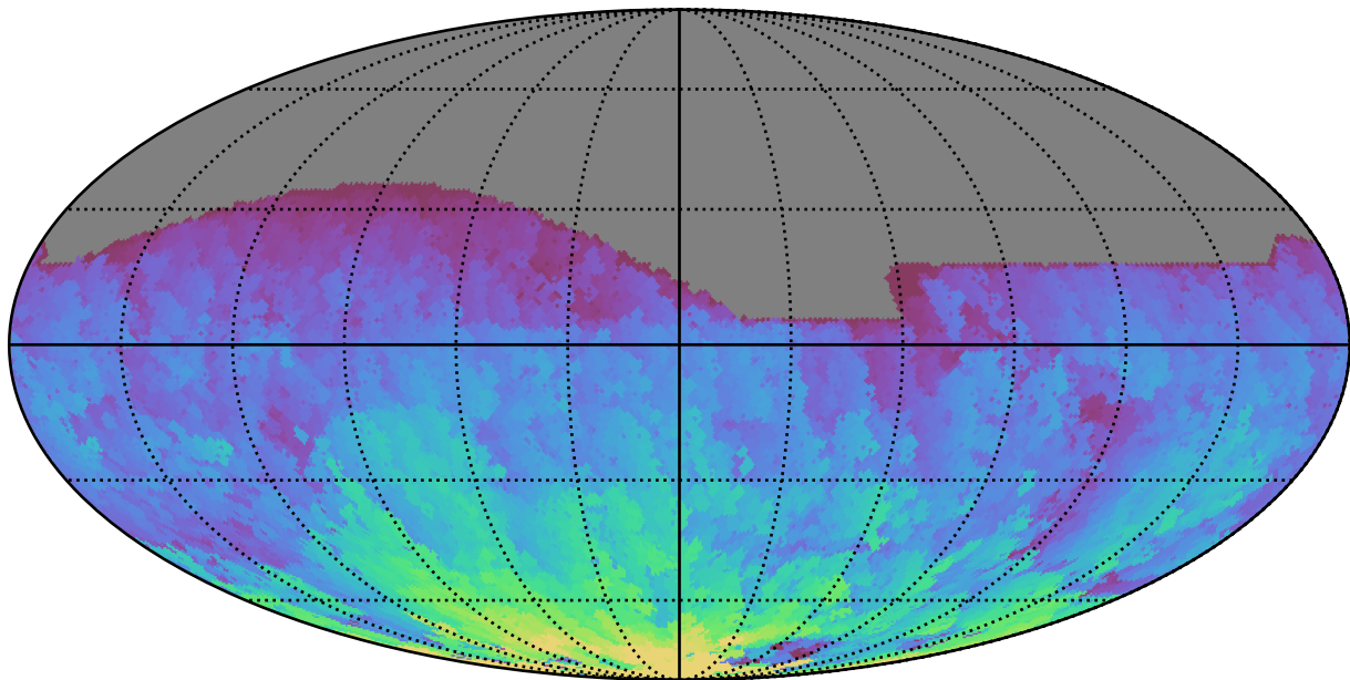
too_elab_r8_d3_ugrizy_v3.4_10yrs All sky r band: Max HA
