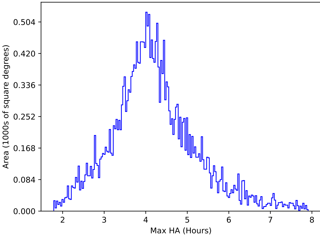
too_elab_r8_d3_ugrizy_v3.4_10yrs All sky r band: Max HA
