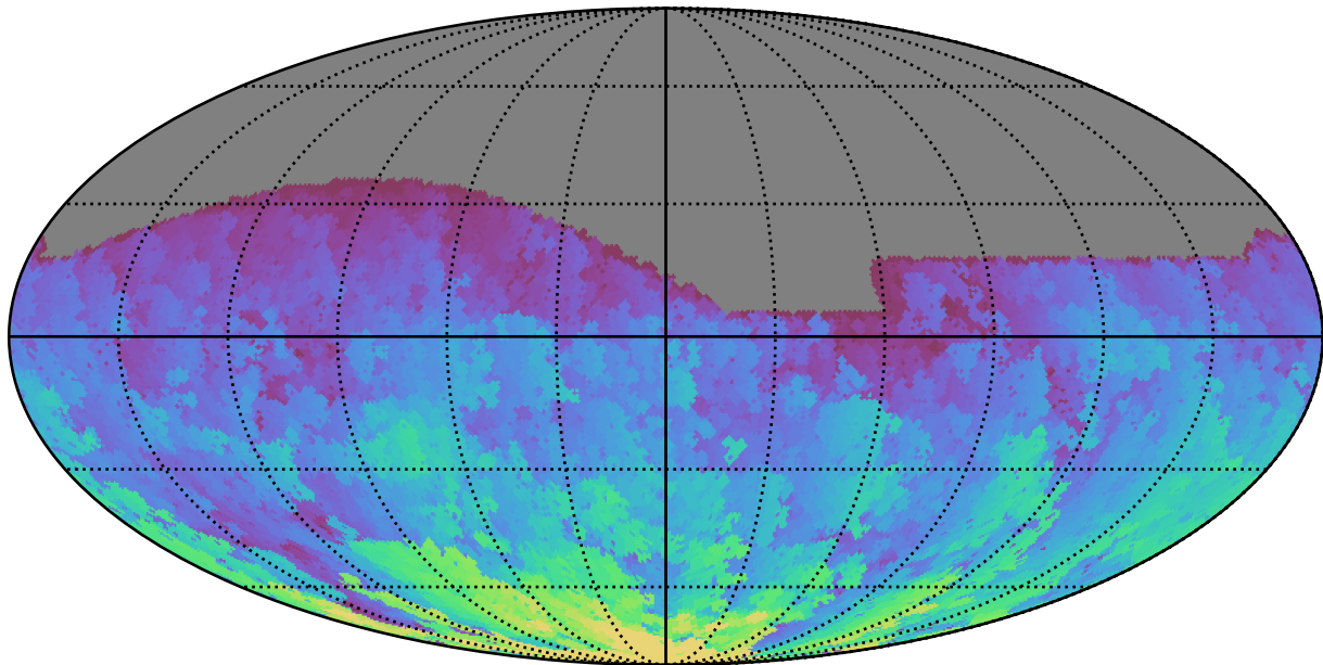
too_elab_r8_d3_ugrizy_v3.4_10yrs All sky g band: Max HA
