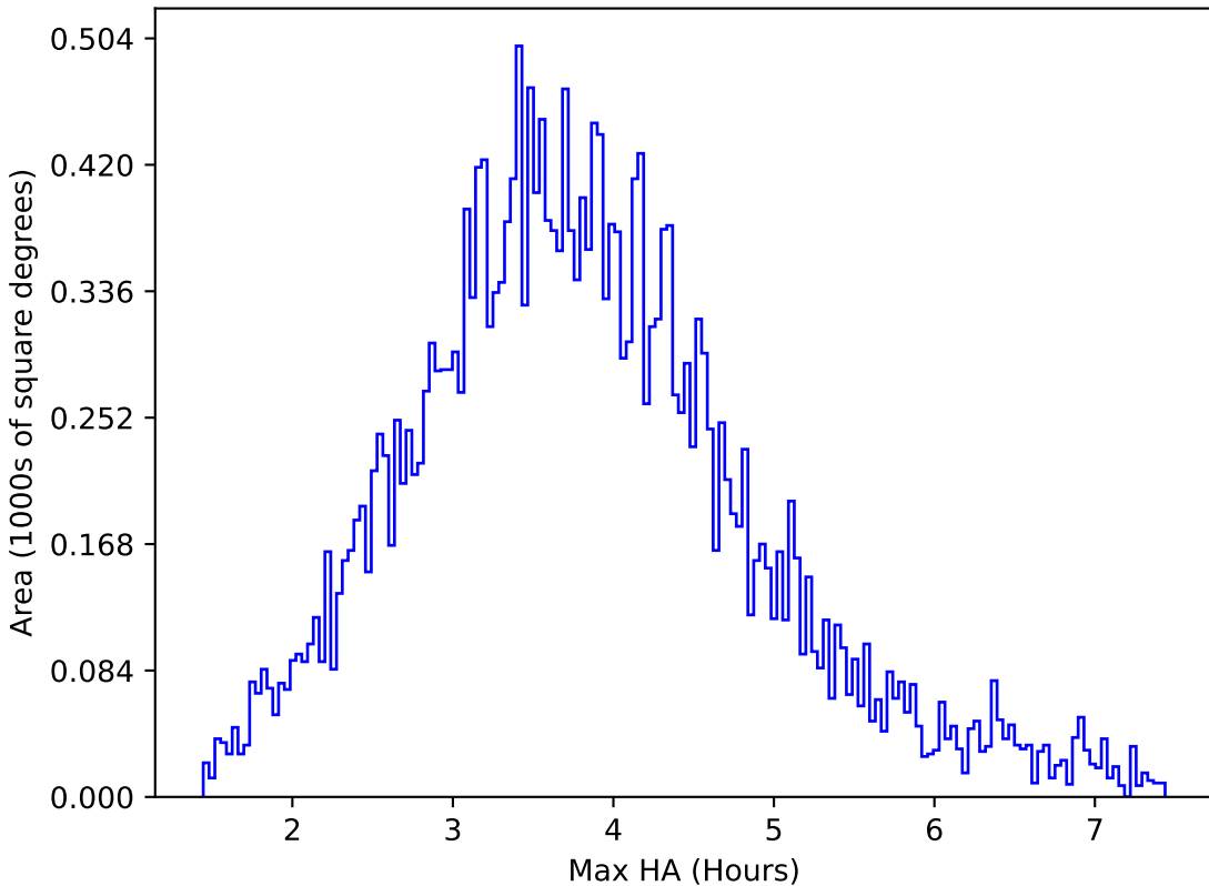
too_elab_r8_d3_ugrizy_v3.4_10yrs All sky g band: Max HA
