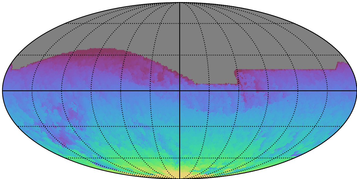
too_elab_r8_d3_ugrizy_v3.4_10yrs All sky all bands: Max HA
