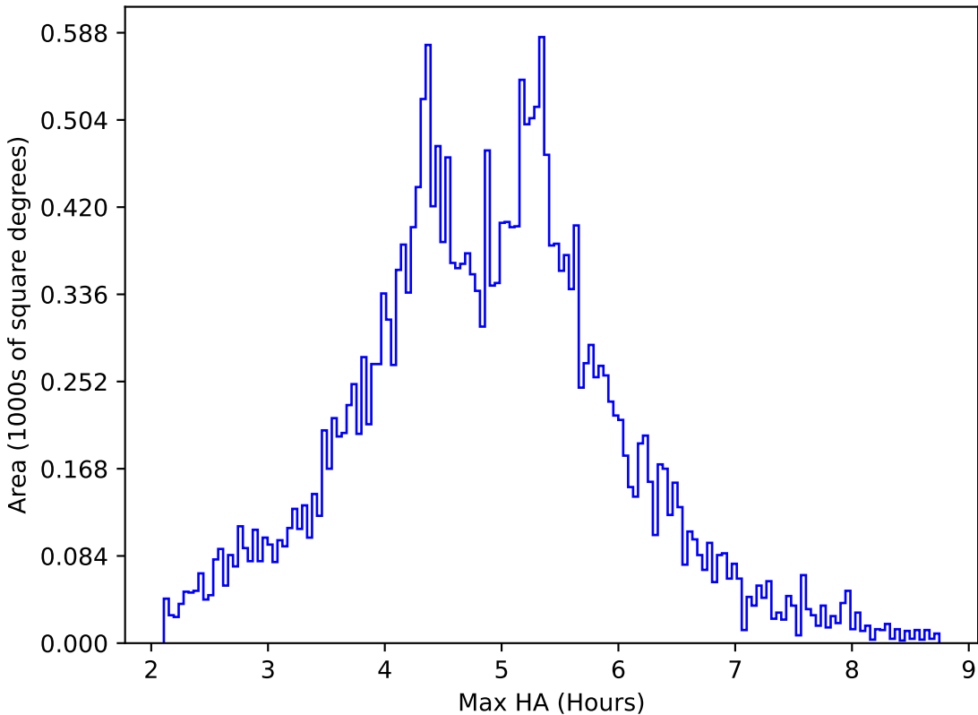
too_elab_r8_d3_ugrizy_v3.4_10yrs All sky all bands: Max HA
