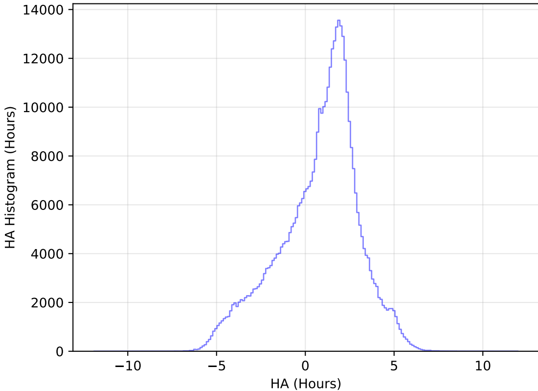
too_elab_r8_d3_ugrizy_v3.4_10yrs WFD z band: HA Histogram
