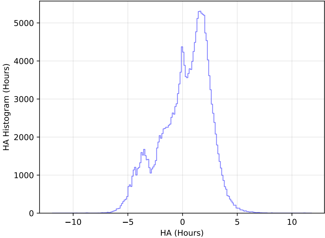
too_elab_r8_d3_ugrizy_v3.4_10yrs WFD g band: HA Histogram
