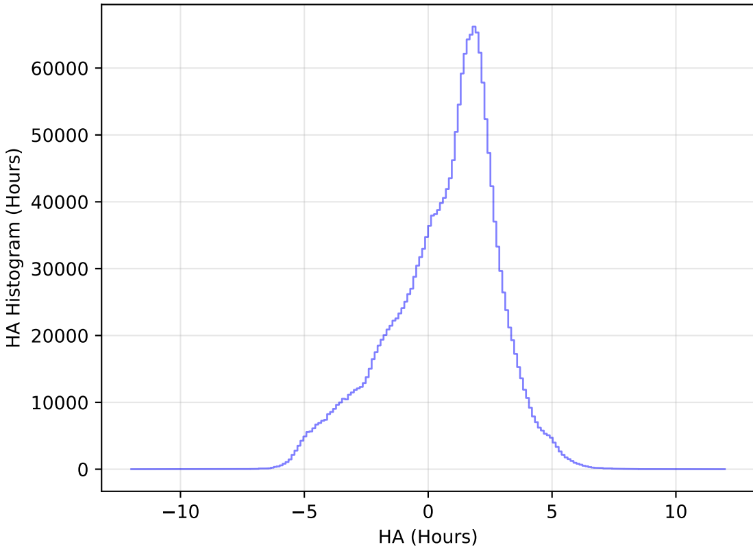
too_elab_r8_d3_ugrizy_v3.4_10yrs WFD all bands: HA Histogram
