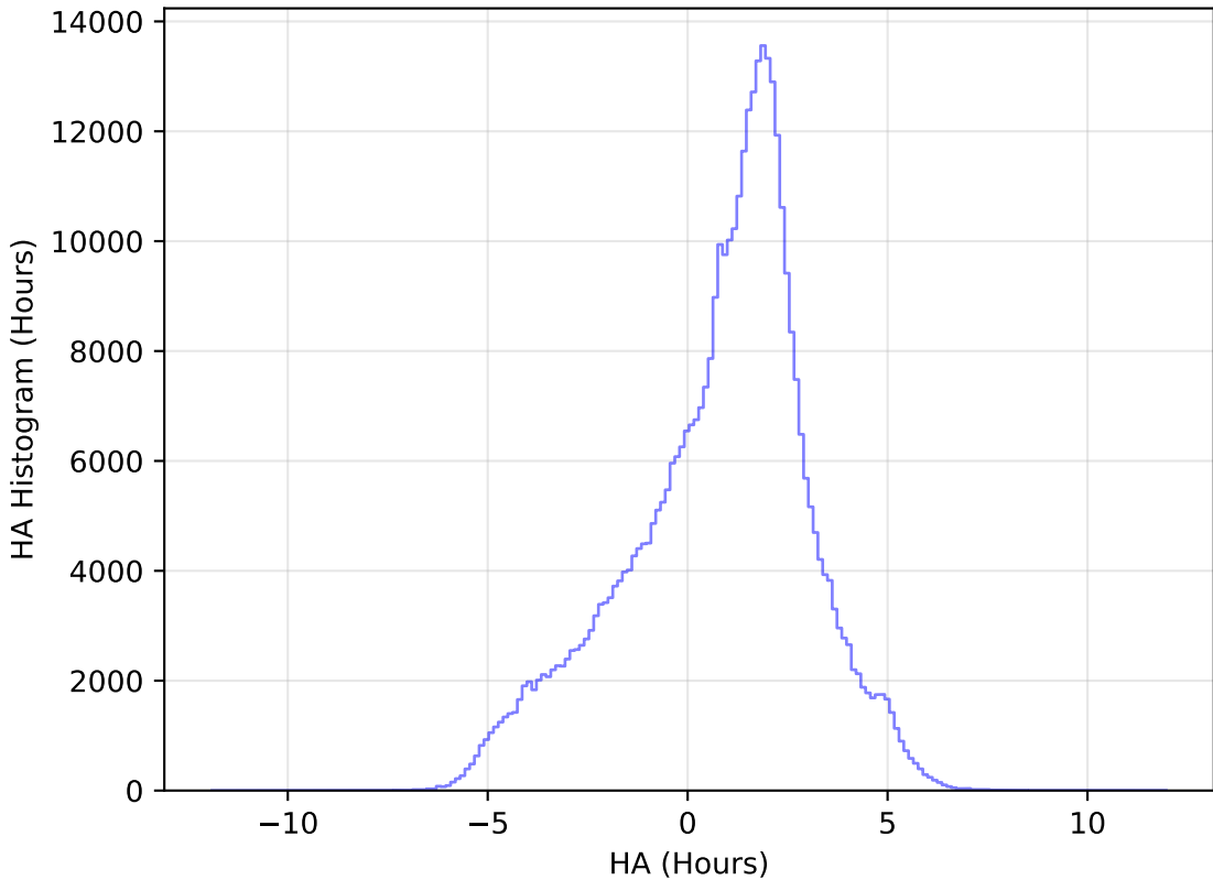
too_elab_r8_d3_ugrizy_v3.4_10yrs All sky z band: HA Histogram
