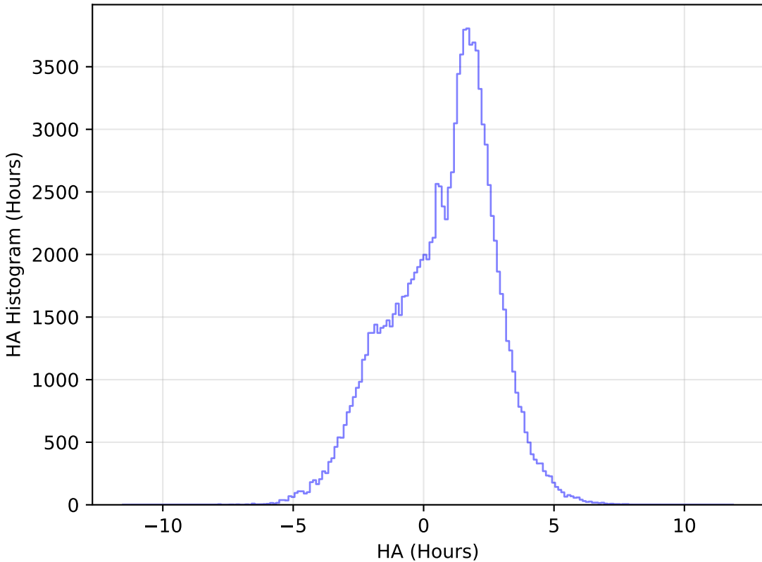
too_elab_r8_d3_ugrizy_v3.4_10yrs All sky u band: HA Histogram
