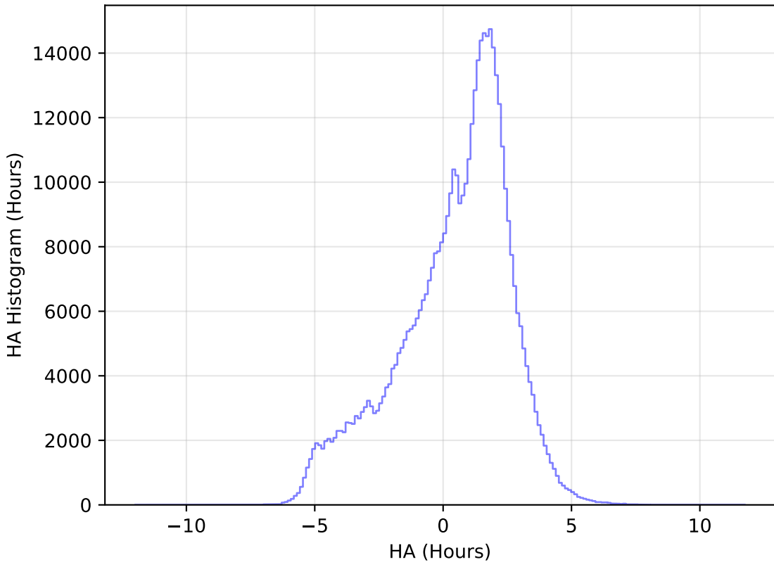
too_elab_r8_d3_ugrizy_v3.4_10yrs All sky r band: HA Histogram
