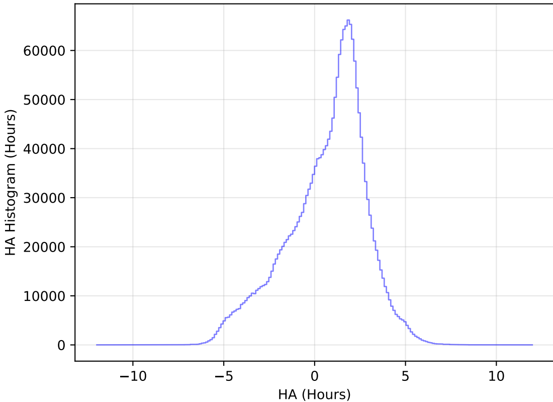
too_elab_r8_d3_ugrizy_v3.4_10yrs All sky all bands: HA Histogram
