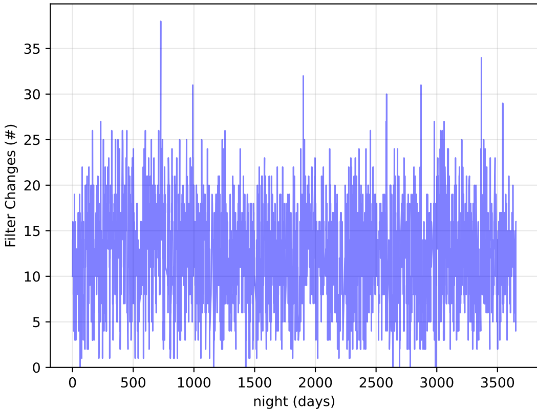
too_elab_r8_d3_ugrizy_v3.4_10yrs Per Night: Filter Changes
