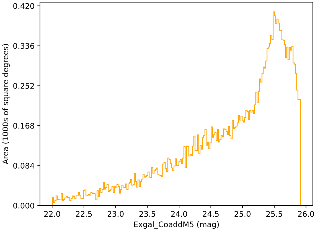
too_elab_r8_d3_ugrizy_v3.4_10yrs Yr 3-4 r band: Exgal_CoaddM5
