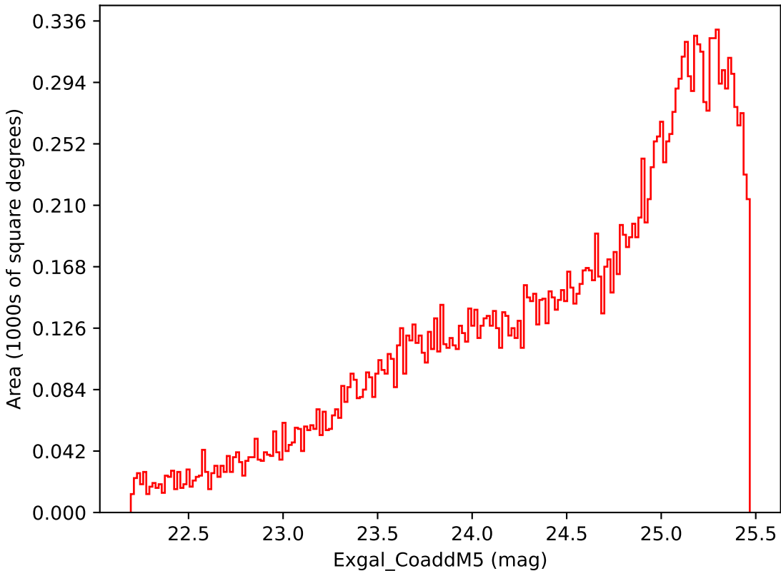
too_elab_r8_d3_ugrizy_v3.4_10yrs Yr 3-4 i band: Exgal_CoaddM5
