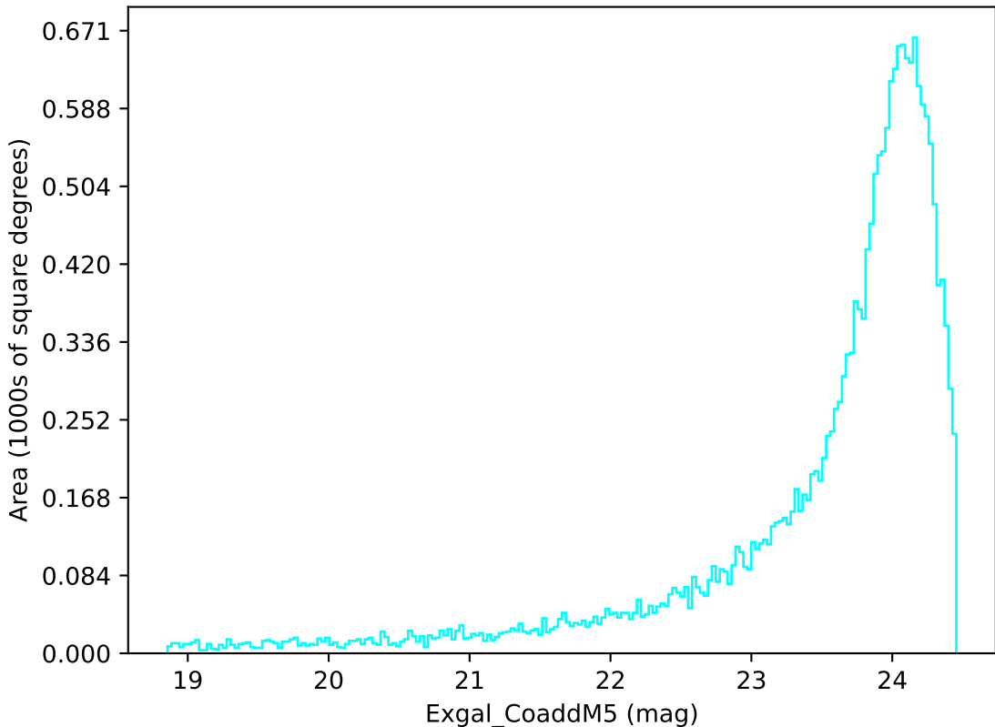
too_elab_r8_d3_ugrizy_v3.4_10yrs Yr 1 u band: Exgal_CoaddM5
