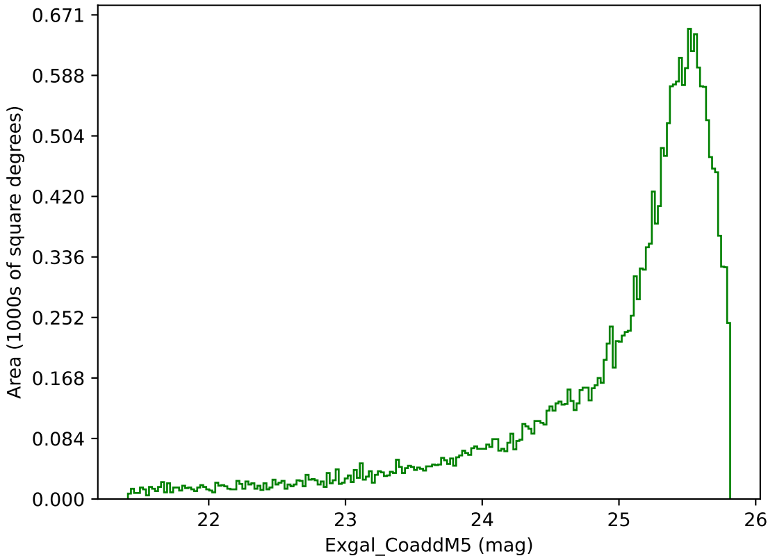
too_elab_r8_d3_ugrizy_v3.4_10yrs Yr 1 g band: Exgal_CoaddM5
