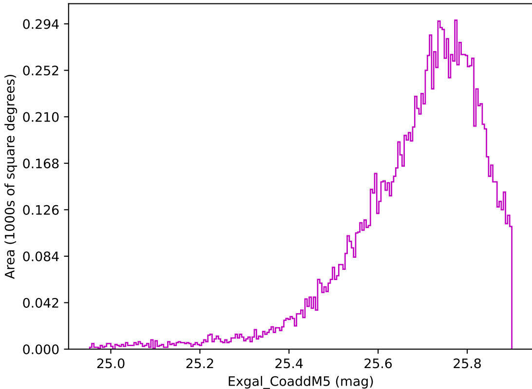
too_elab_r8_d3_ugrizy_v3.4_10yrs WFD z band: Exgal_CoaddM5
