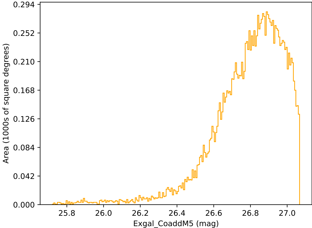
too_elab_r8_d3_ugrizy_v3.4_10yrs WFD r band: Exgal_CoaddM5
