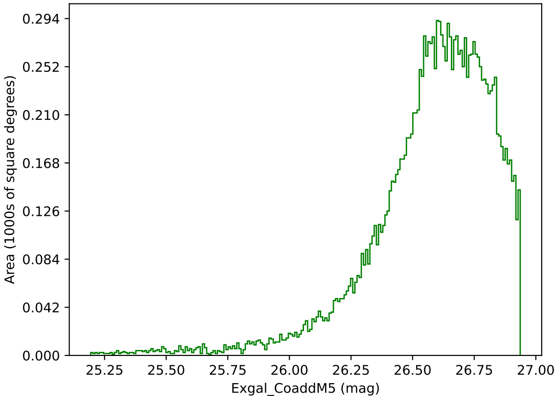
too_elab_r8_d3_ugrizy_v3.4_10yrs WFD g band: Exgal_CoaddM5
