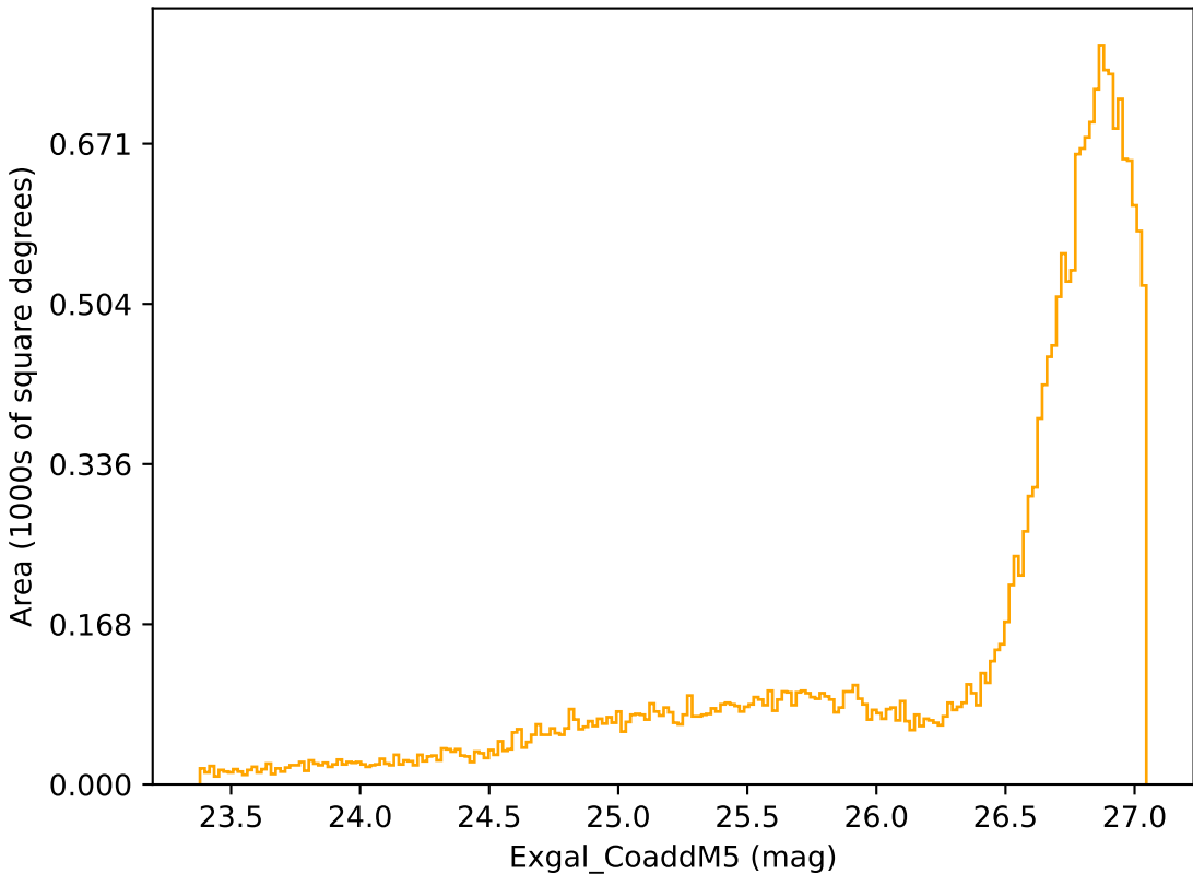
too_elab_r8_d3_ugrizy_v3.4_10yrs All sky r band: Exgal_CoaddM5
