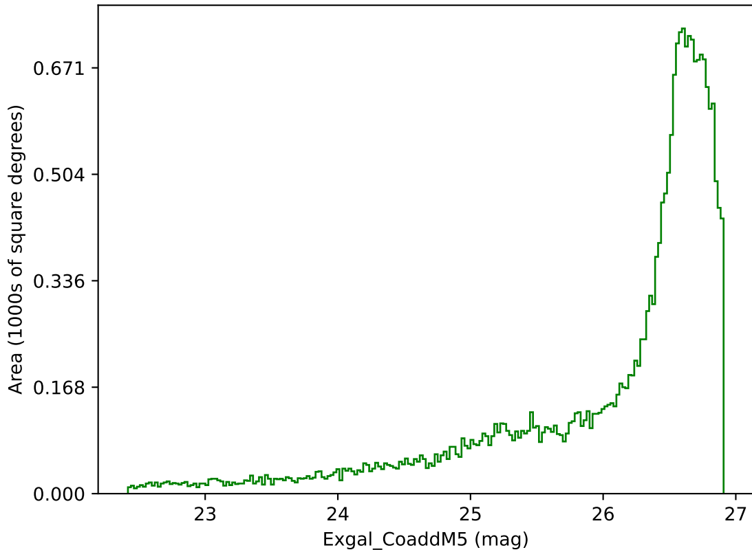
too_elab_r8_d3_ugrizy_v3.4_10yrs All sky g band: Exgal_CoaddM5
