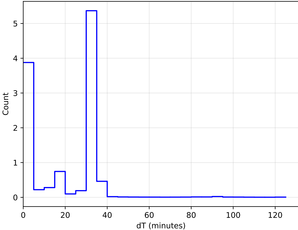
too_elab_r8_d3_ugrizy_v3.4_10yrs WFD: DeltaT Histogram 1e6
