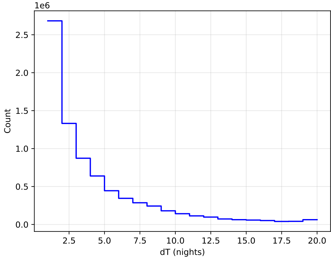
too_elab_r8_d3_ugrizy_v3.4_10yrs WFD all bands: DeltaNight Histogram
