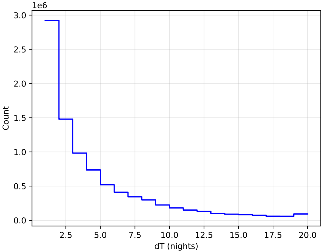
too_elab_r8_d3_ugrizy_v3.4_10yrs All sky all bands: DeltaNight Histogram
