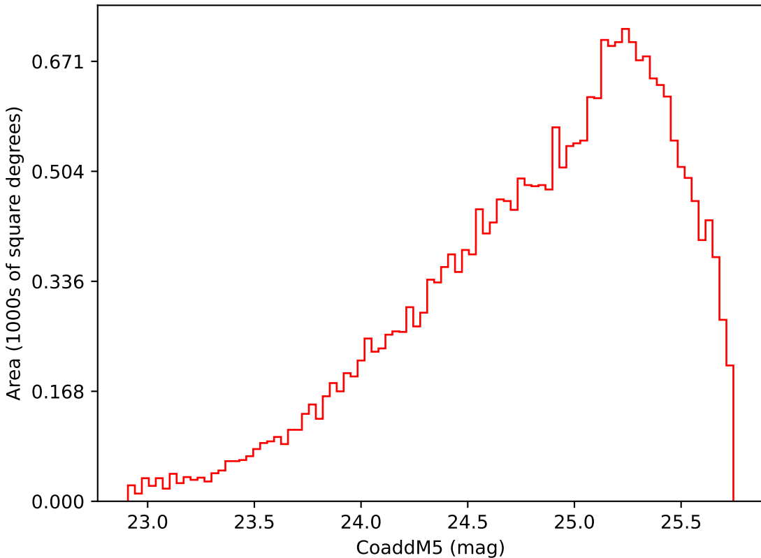
too_elab_r8_d3_ugrizy_v3.4_10yrs Yr 3-4 i band: CoaddM5
