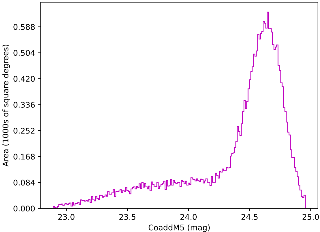
too_elab_r8_d3_ugrizy_v3.4_10yrs Yr 1 z band: CoaddM5
