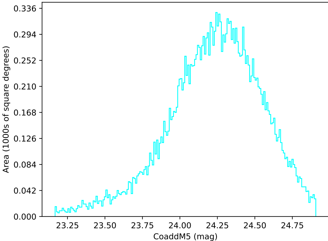
too_elab_r8_d3_ugrizy_v3.4_10yrs Yr 1 u band: CoaddM5
