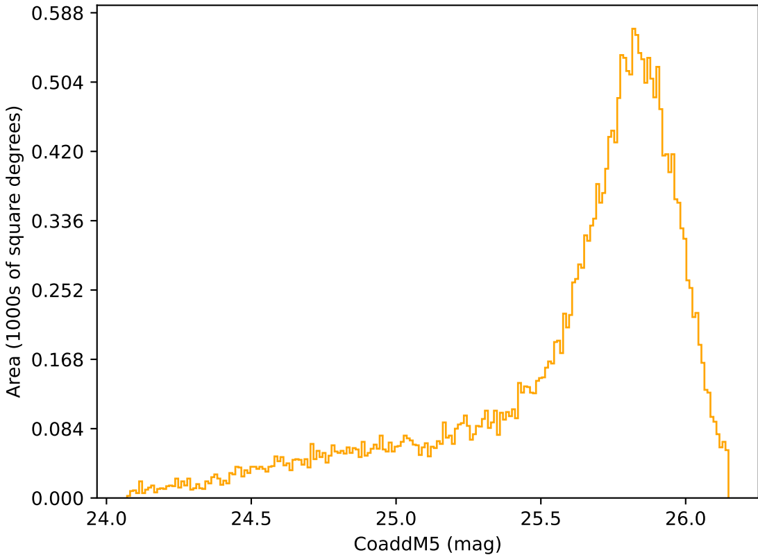
too_elab_r8_d3_ugrizy_v3.4_10yrs Yr 1 r band: CoaddM5
