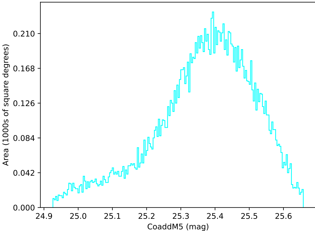
too_elab_r8_d3_ugrizy_v3.4_10yrs WFD u band: CoaddM5
