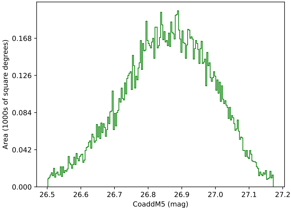
too_elab_r8_d3_ugrizy_v3.4_10yrs WFD g band: CoaddM5
