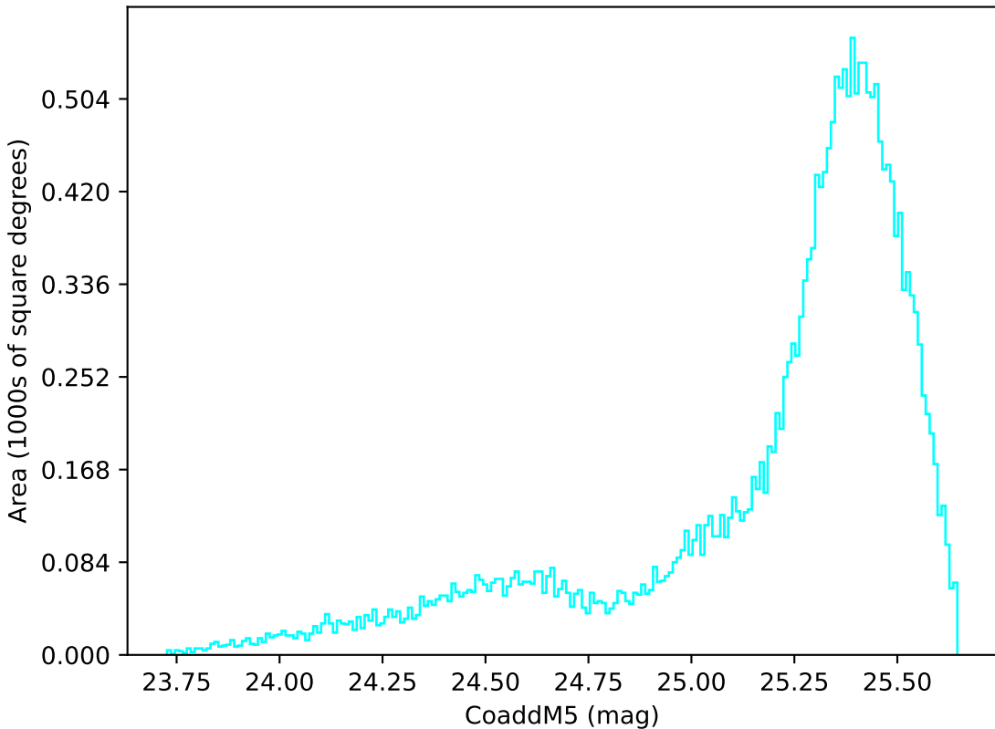
too_elab_r8_d3_ugrizy_v3.4_10yrs All sky u band: CoaddM5
