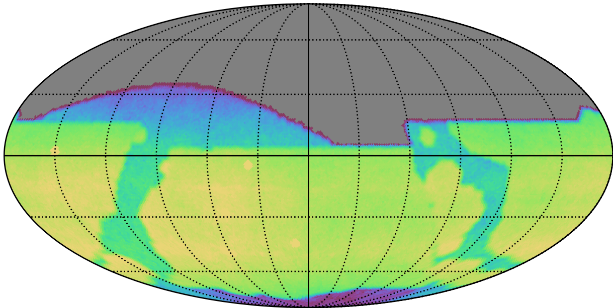
too_elab_r8_d3_ugrizy_v3.4_10yrs All sky r band: CoaddM5
