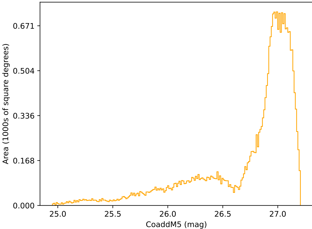
too_elab_r8_d3_ugrizy_v3.4_10yrs All sky r band: CoaddM5
