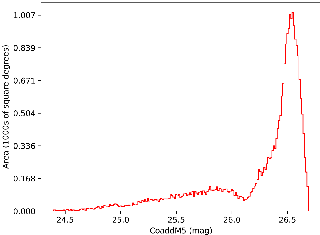
too_elab_r8_d3_ugrizy_v3.4_10yrs All sky i band: CoaddM5
