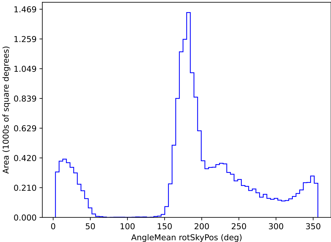
too_elab_r8_d3_ugrizy_v3.4_10yrs WFD g band: AngleMean rotSkyPos
