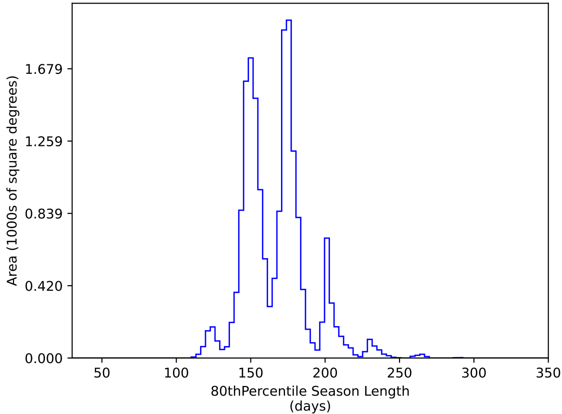
too_elab_r8_d3_ugrizy_v3.4_10yrs WFD y band: 80thPercentile Season Length
