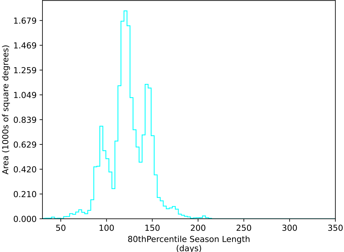
too_elab_r8_d3_ugrizy_v3.4_10yrs WFD u band: 80thPercentile Season Length
