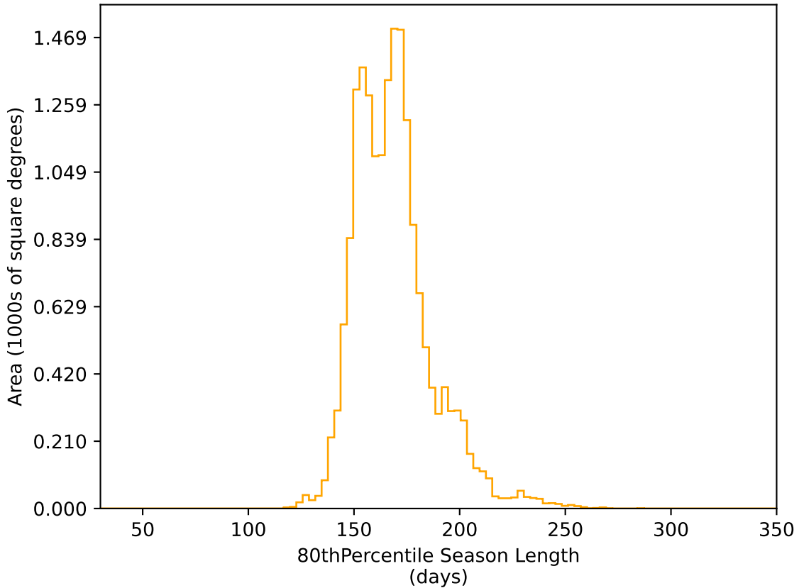
too_elab_r8_d3_ugrizy_v3.4_10yrs WFD r band: 80thPercentile Season Length
