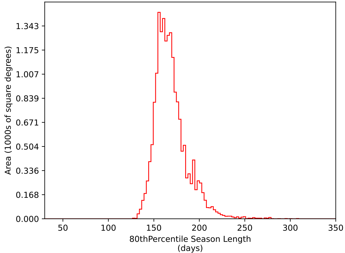
too_elab_r8_d3_ugrizy_v3.4_10yrs WFD i band: 80thPercentile Season Length
